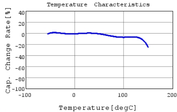
RHEL82A103K0K1H03B C-Temp. capchange, DCOV,
