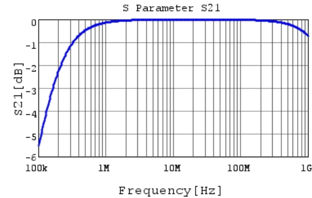
RHEL82A103K0K1H03B S21 DCOV, 25degC
