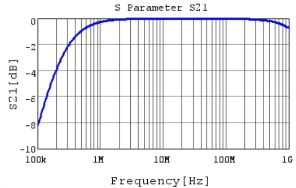
RHEL82A682K0K1H03B S21 DCOV, 25degC
