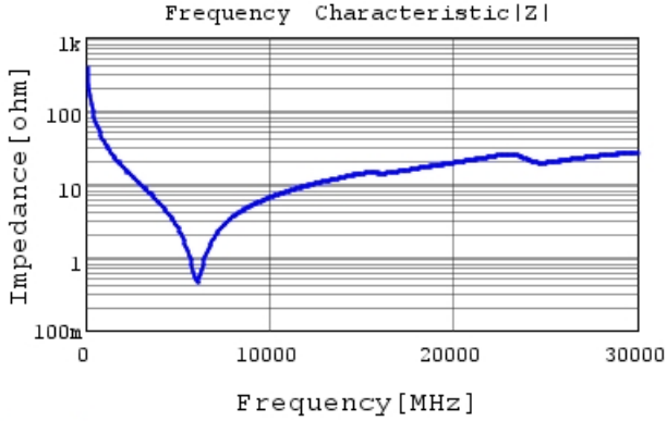
GRM0225C1H4R1WA03 |Z| DCOV, 25degC
