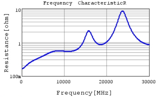
GRM0225C1H4R1WA03 R DCOV, 25degC
