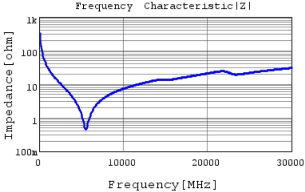
GRM0225C1H4R8BA03 |Z| DCOV,25degC
