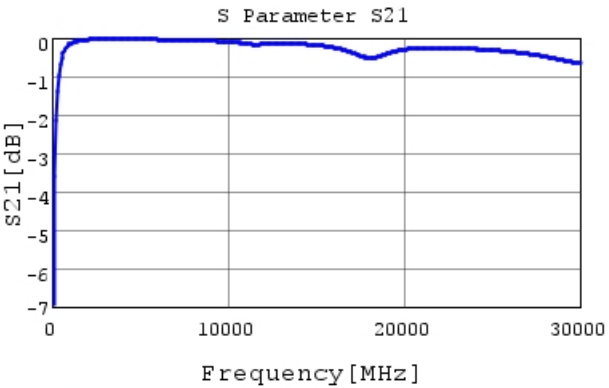
GRM0225C1H8R0WA03 S21 DCOV, 25degC
