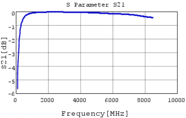
GRM1552C1H9R7BA01 S21 DCOV, 20degC
