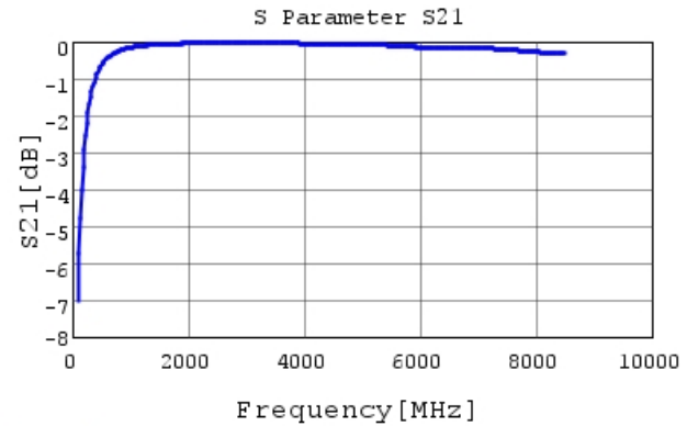
GRM1552C2A7R9WA01 S21 DCOV, 20degC
