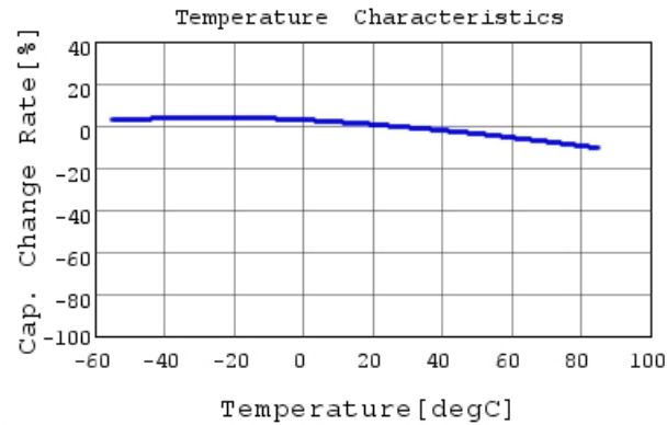
GRT188R61A105KE01 C-Temp. capchange, DC0.0V,
