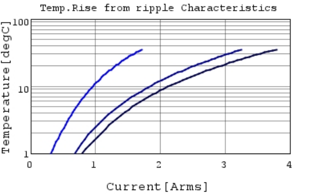
GRT188R61A105KE01 Temp.rise 100kHz
