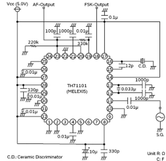
Measurement Circuit
