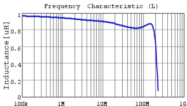
1225AS-H-1R0N L
