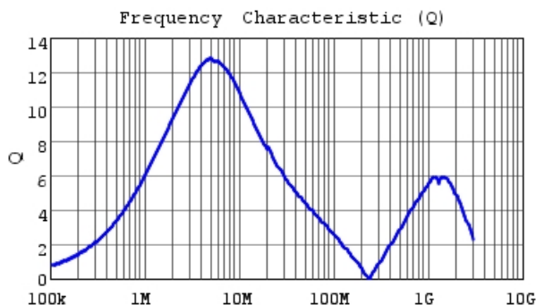
1225AS-H-1R0N Q
