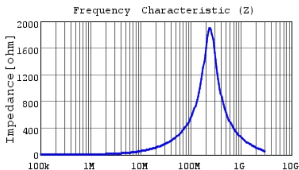
1225AS-H-1R0N |Z|
