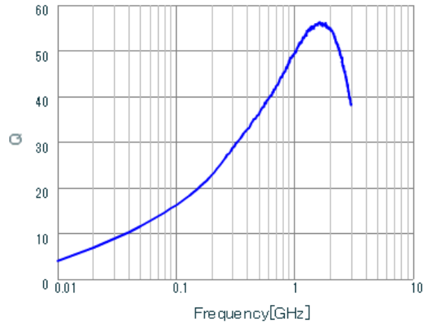
LQG15WZ9N5G02 Q.
