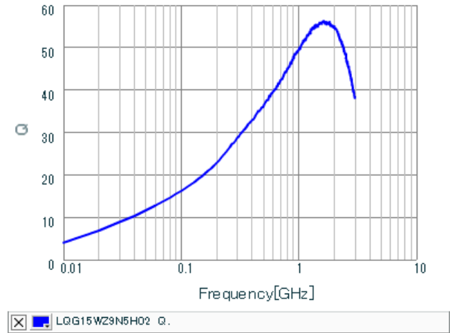
Q-Frequency Characteristics
