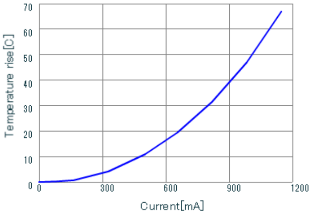
LQH2HPN100MJR DT_Current
