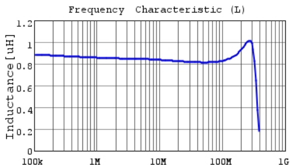
LQH32NH1R0M23 L
