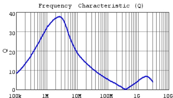
LQH32NH1R0M23 Q
