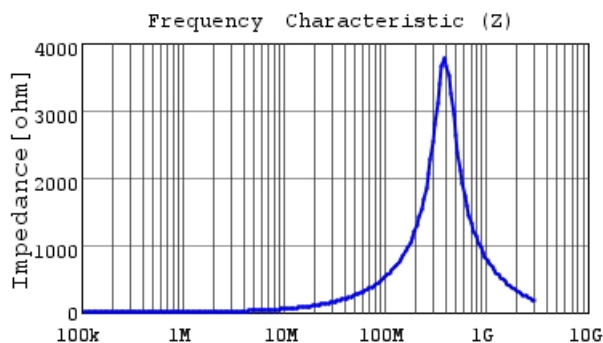
LQH32NH1R0M23 |Z|
