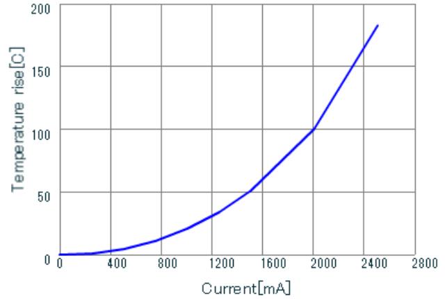
LQH3NPN100MMR DT_Current
