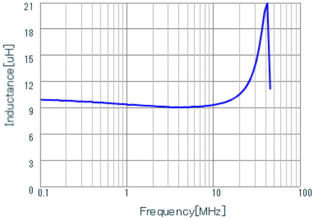
LQH3NPN100MMR L
