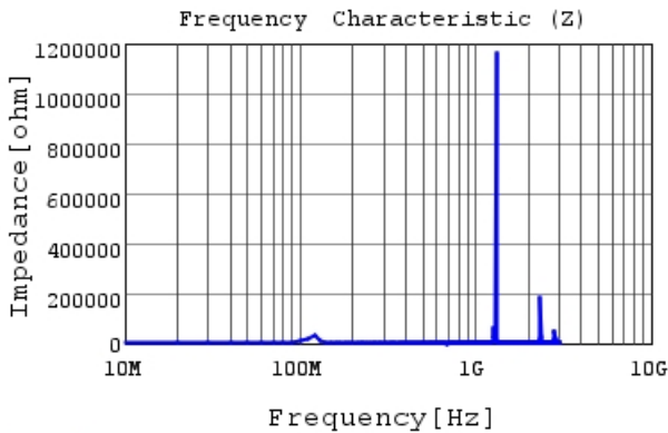
LQW2UAS3R3J00 |Z|
