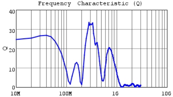
LQW2UAS3R3J00 Q
