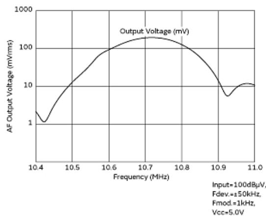
Frequency Characteristics
