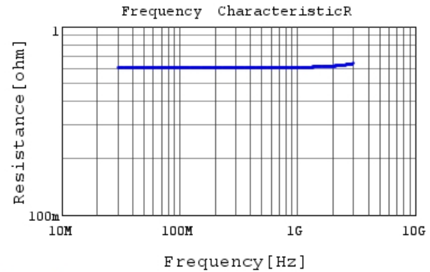
RCE5C1H1R0C0K1H03B R DCOV,25degC
