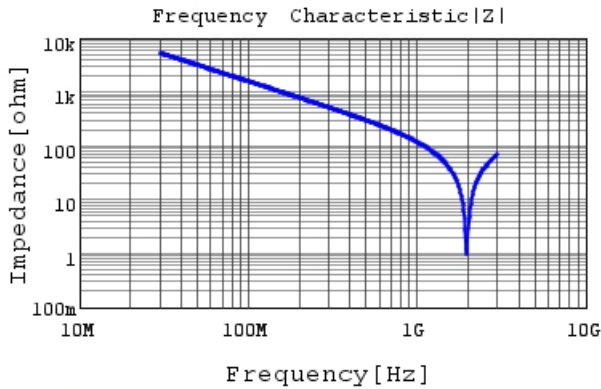
RCE5C1H1R0C0K1H03B |Z| DCOV,25degC
