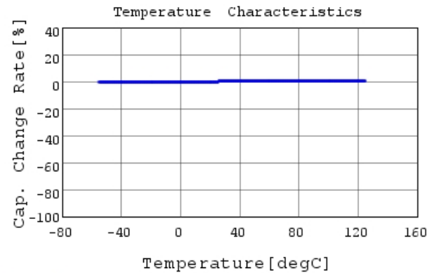
RCE5C1H1R0C0K1H03B C-Temp. capchange, DCOV,
