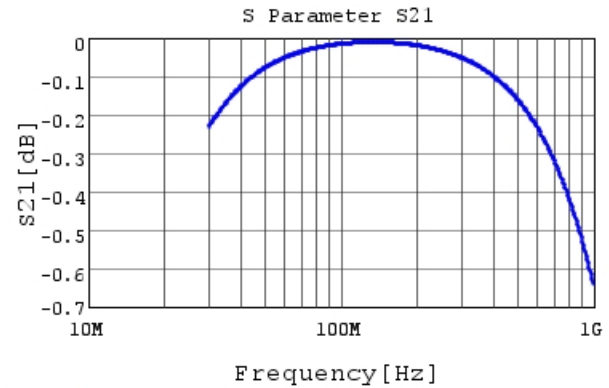
RHE5G1H221J0K1H03B S21 DCOV, 25degC
