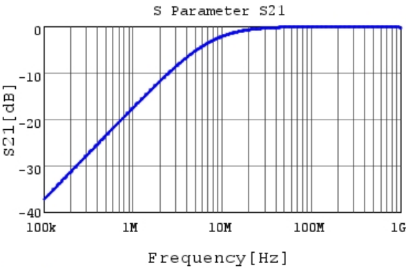
RHEL81H221K0A2H03B S21 DCOV, 25degC
