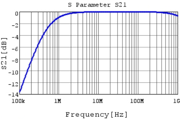
RHEL82A332K0K1H03B S21 DCOV, 25degC
