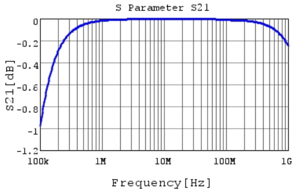
RHEL82A333K1DBH03A S21 DCOV, 25degC
