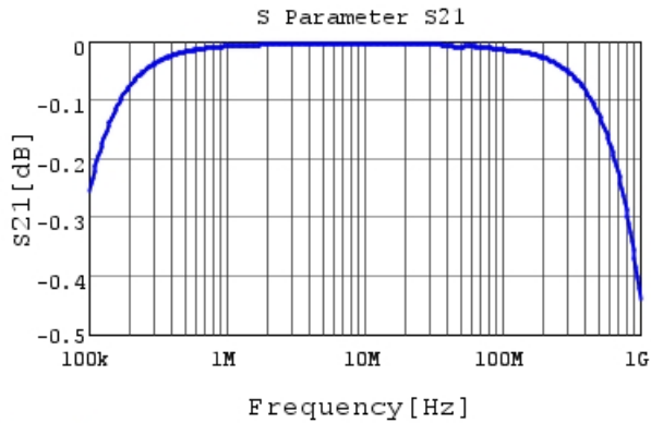
RHEL82A683K1M1H03A S21 DCOV, 25degC
