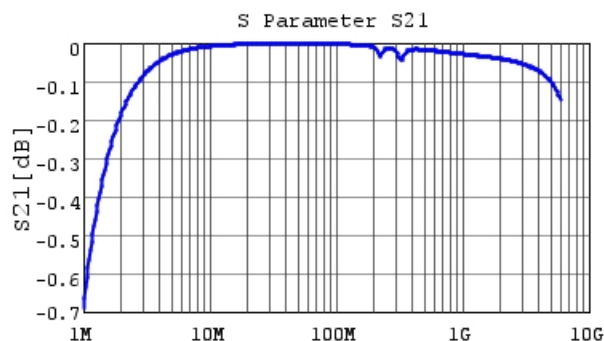
■ GCM1885C1H392JA16 S21 DCOV, 25degC
