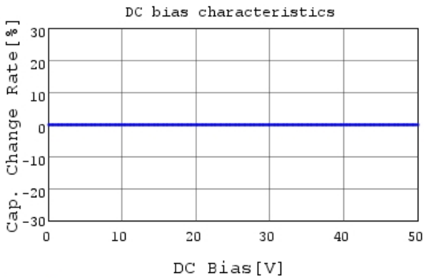
GRM0225C1H2R2BA03 C-DC bias capchange, 25.0C
