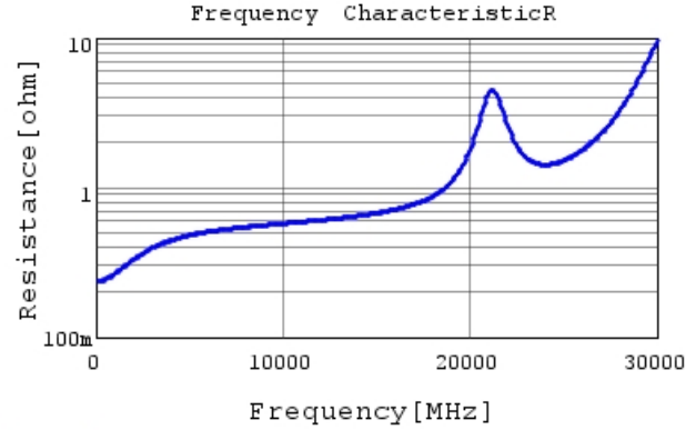
GRM0225C1H2R2BA03 R DCOV, 25degC
