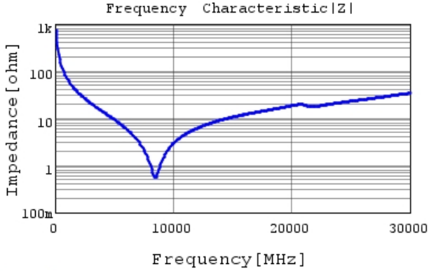
GRM0225C1H2R2BA03 |Z| DCOV, 25degC
