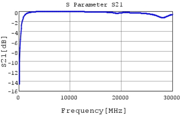
GRM0225C1H3R0WA03 S21 DCOV, 25degC
