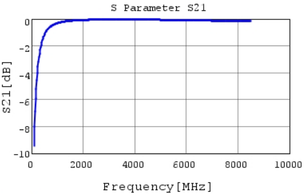
GRM0335C1H5R7DA01 S21 DCOV, 25degC
