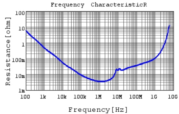
GRM21BR60J225KA01 R DCOV, 25degC
