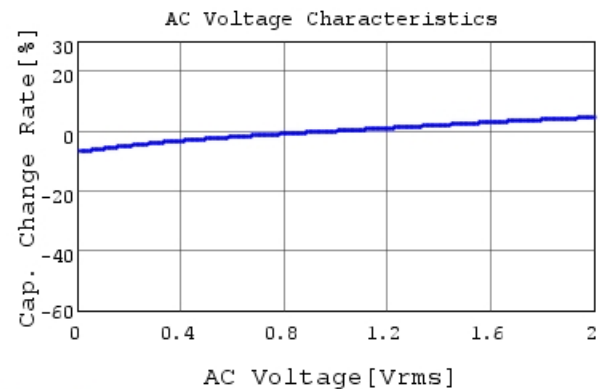
GRM21BR60J225KA01 C-AC Voltage capchange, D
