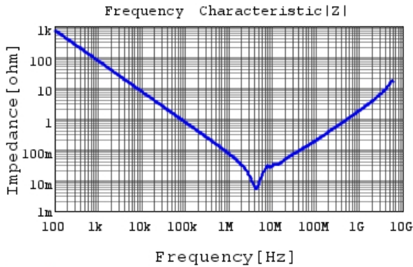
GRM21BR60J225KA01 |Z| DCOV, 25degC
