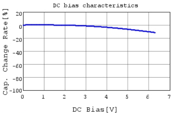
GRM21BR60J225KA01 C-DC bias capchange, 25.0C
