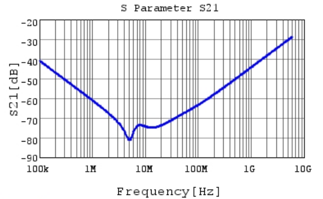
NFM18HC106D0G3 S21 DCOV, 25degC, Feedthrough
