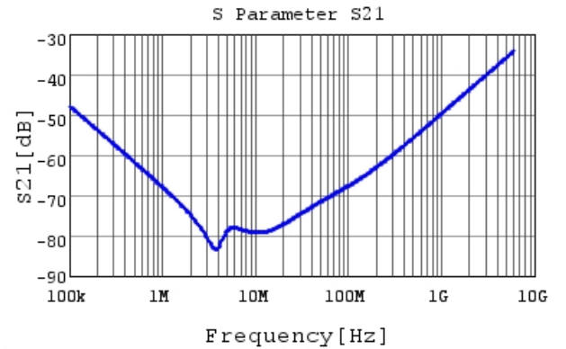
NFMJMPC226D0E3 S21 DCOV, 25degC, Feedthrough
