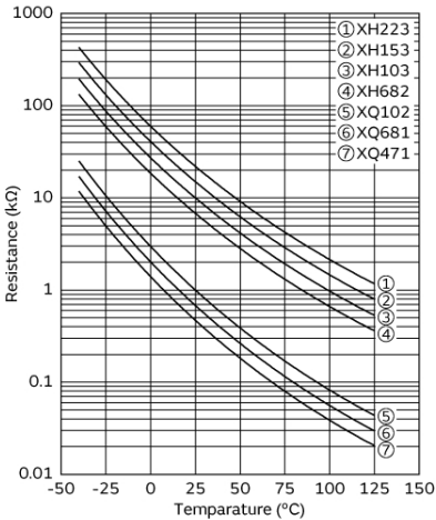
Resistance-Temperature Characteristics
