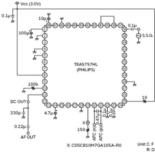
Measurement Circuit
