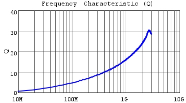
LQP02TN0N8C02 Q
