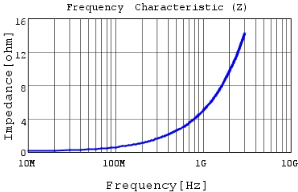
LQP02TN0N8C02 |Z|
