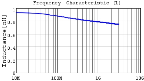
LQP02TN0N8C02 L
