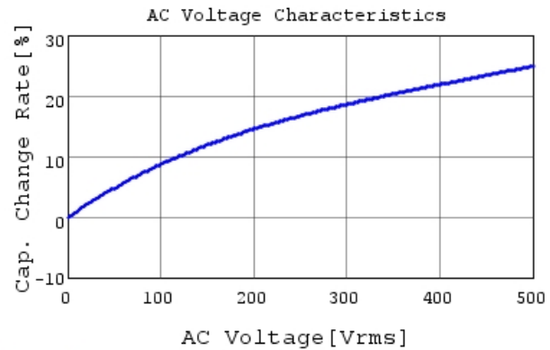
DE1B3RB471KN4AR01F C-AC Voltage capchange, 1
