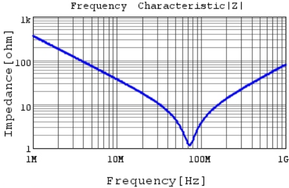
DE1B3RB471KN4AR01F |Z| DCOV, 20degC
