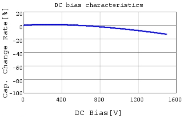
DE1B3RB471KN4AR01F C-DC bias capchange, 20.0
