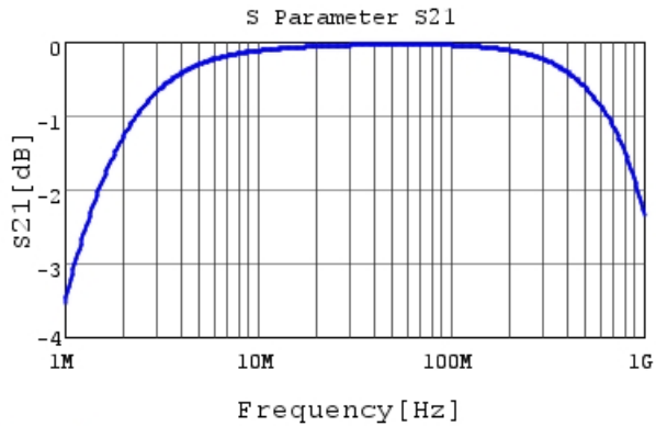
DE1E3RA152MJ4BN01F S21 DCOV, 20degC
