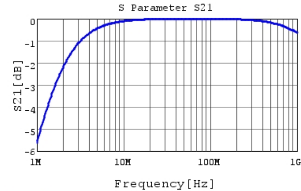
RHE5G1H102J0M1H03A S21 DCOV, 25degC
