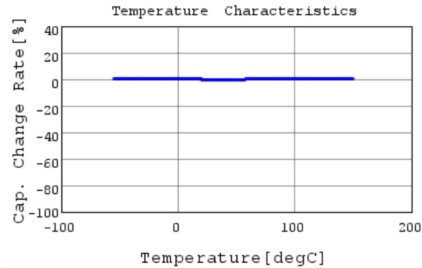
RHE5G1H102J0M1H03A C-Temp. capchange, DCOV,
