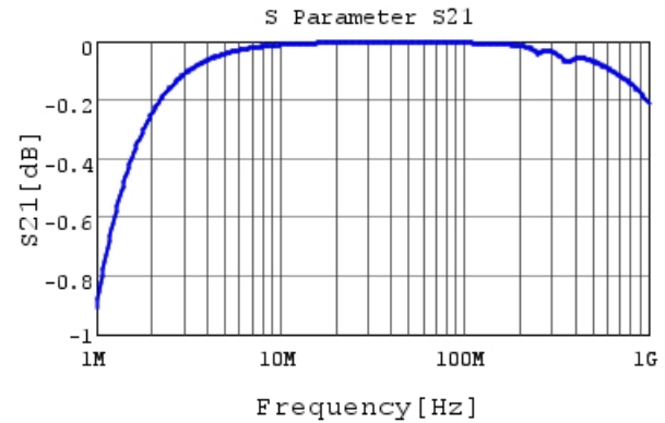
RHE5G1H332J0A2H03B S21 DCOV, 25degC
