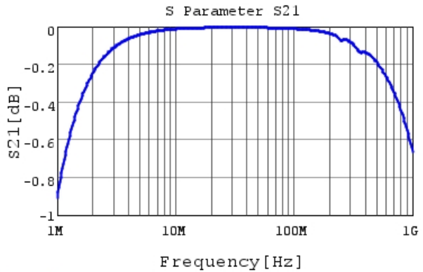
RHE5G1H332J0M1H03A S21 DCOV, 25degC
