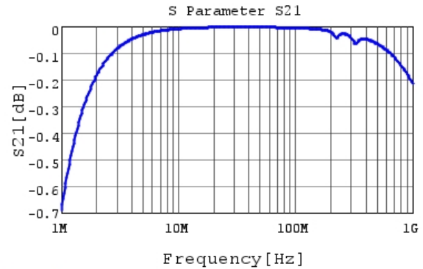
RHE5G1H392J0DBH03A S21 DCOV, 25degC
