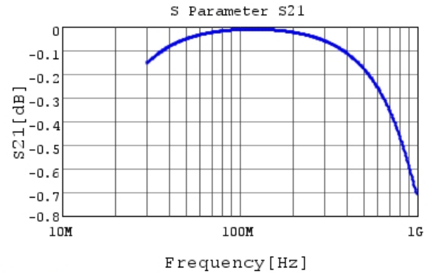
RHE5G2A271J0K1H03B S21 DC0V, 25degC
