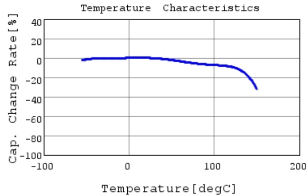
RHEL81H154K1M1H03A C-Temp. capchange, DCOV,
