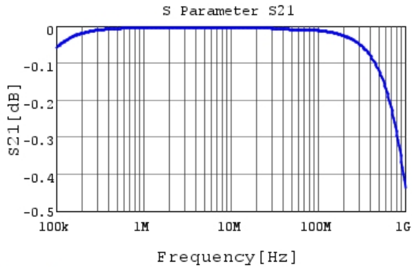
RHEL81H154K1M1H03A S21 DCOV, 25degC
