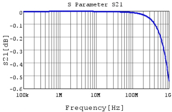
RHEL81H684K2K1H03B S21 DCOV, 25degC
