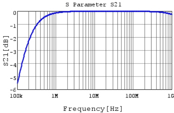
RHEL82A103K0A2H03B S21 DCOV, 25degC
