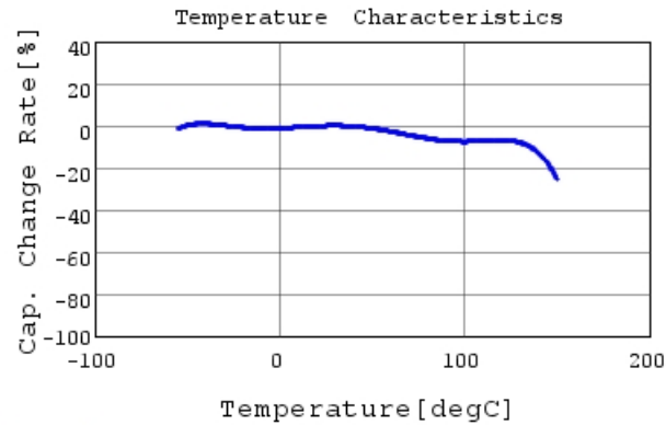
RHEL82A103K0A2H03B C-Temp. capchange, DCOV,
