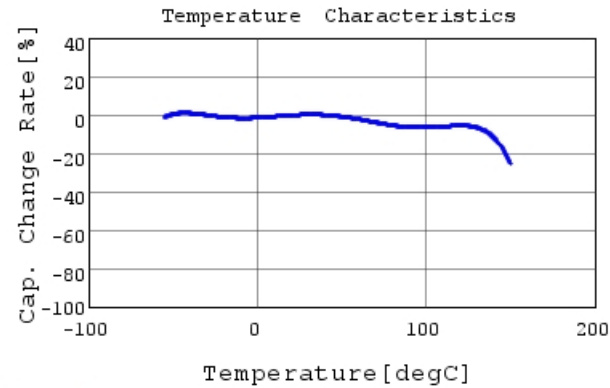
RHEL82A104K1M1H03A C-Temp. capchange, DCOV,
