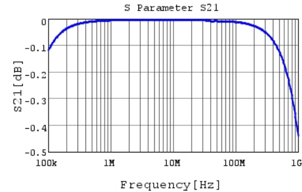
RHEL82A104K1M1H03A S21 DCOV, 25degC
