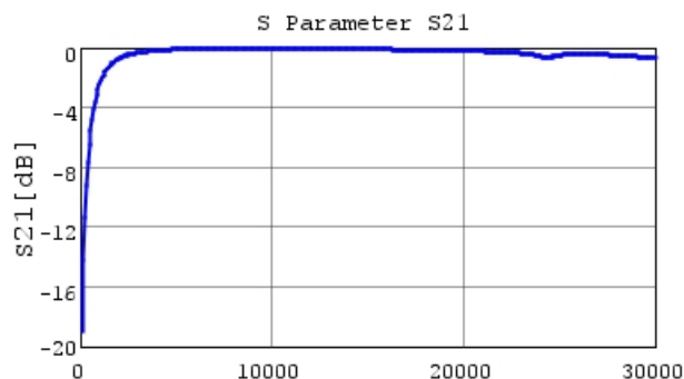
GRM0224C1H1R8CA03 S21 DCOV, 20degC
