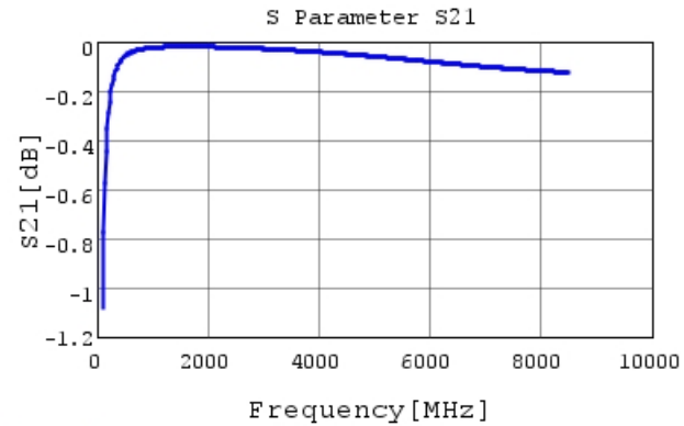
GRM0225C1H300JA02 S21 DCOV, 25degC
