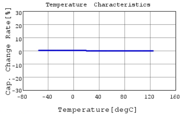
GRM0332C2A7R2WA01 C-Temp. capchange, DCOV, 1
