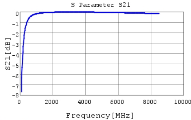
GRM0332C2A7R2WA01 S21 DCOV, 20degC
