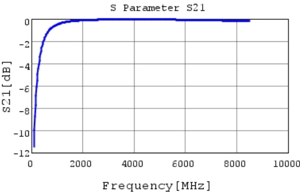
GRM0335C2A4R4WA01 S21 DCOV, 25degC
