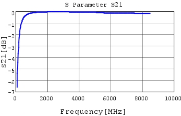
GRM1555C2A8R4WA01 S21 DCOV, 25degC
