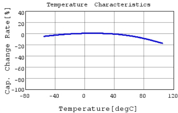
GRM155C80G224KE01 C-Temp. capchange, DC0.0V,
